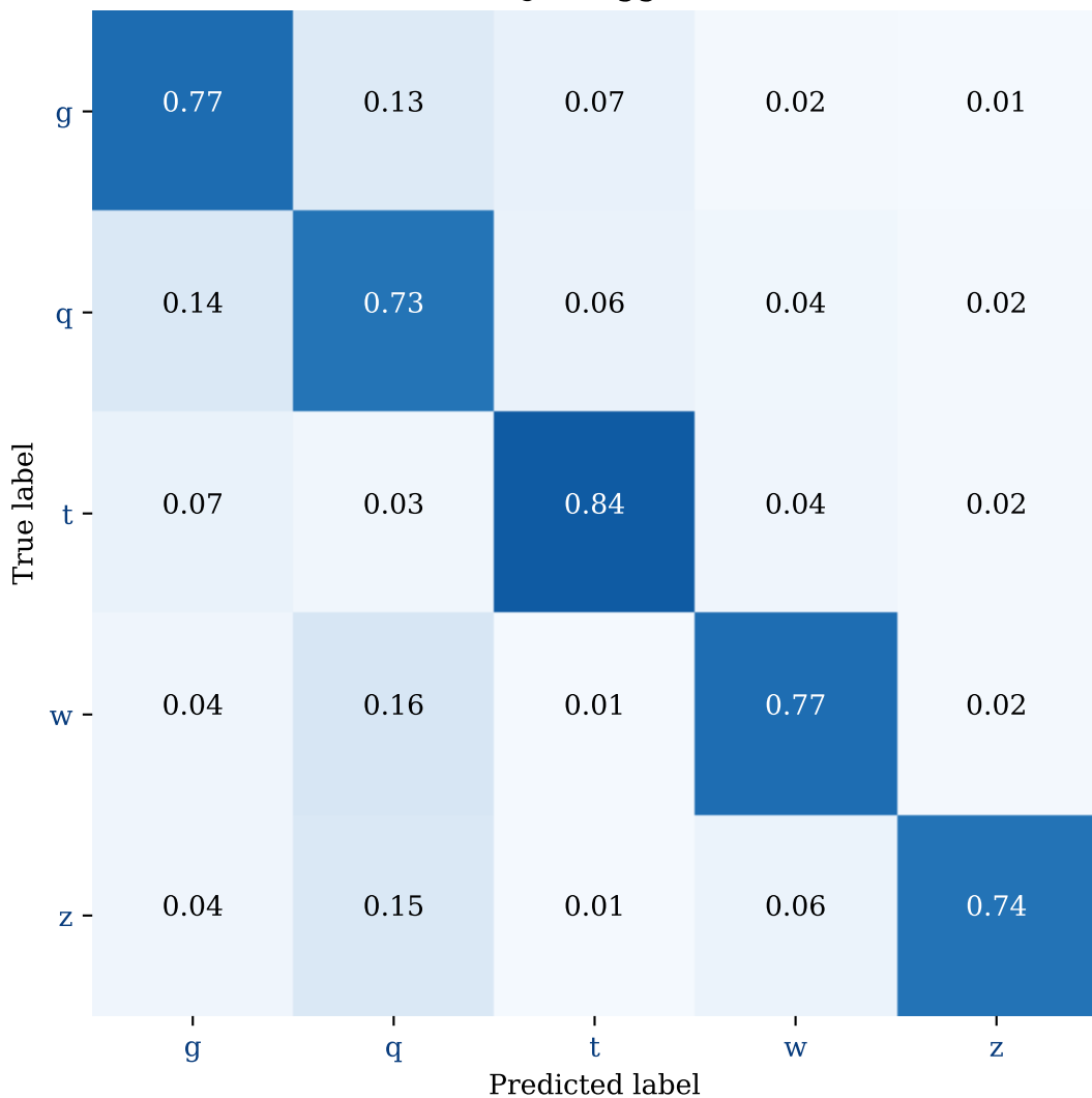
Confusion Matrix of a Jet-tagger Classifier (baseline)
